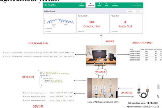
Fig.5 Experimental setup of LoRa WAN Soil moisture sensor
