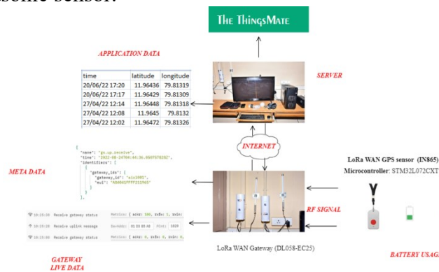
Fig.9 Experimental setup of LoRa WAN GPS sensor
