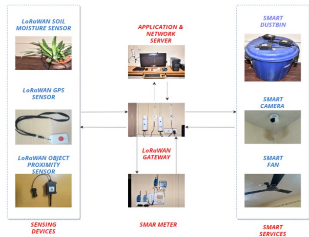
Fig.2 Overall laboratory setup
