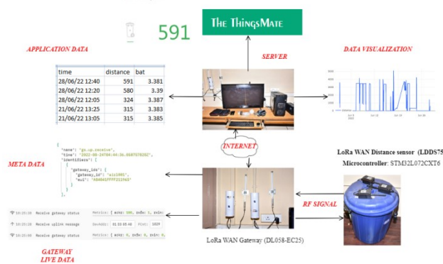
Fig.6 Experimental setup of a LoRa WAN ultrasonic sensor
