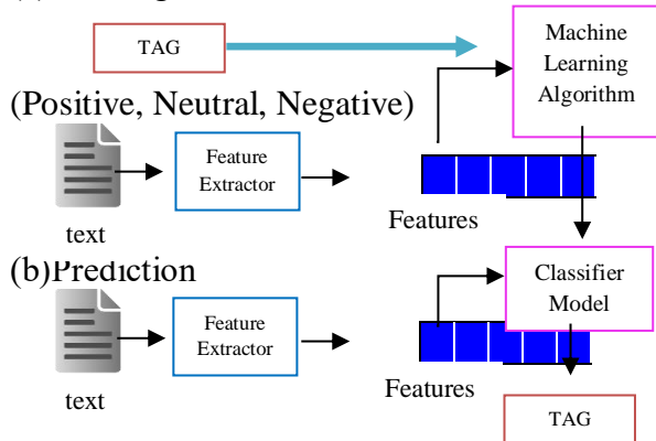
Fig. 2 : Natural Language Processing Work Flow
