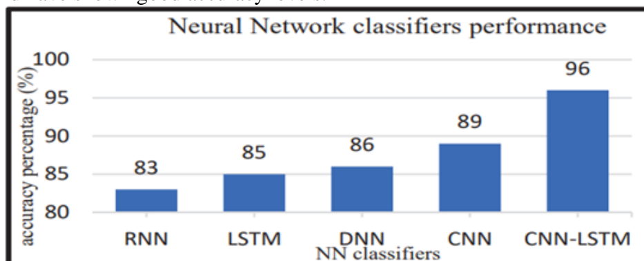
Fig. 5 : The comparison of Neural Network classifiers performance
