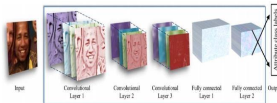
Fig 2: Architecture of used CNN
