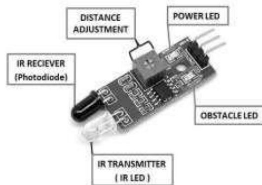
Fig.3 IR Transmitter and Receiver Sensor
